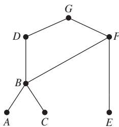
FIGURE 10 The Hasse Diagram for Seven Tasks.
